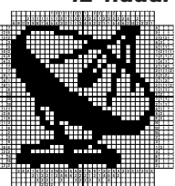
42 Radar
